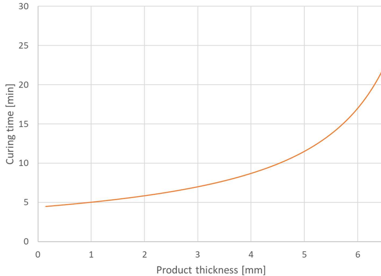
Curing times for the vulcanization of rubber plates, Auma type 10 (Rotocure machine with heating drum diameter = 1.0 m)
