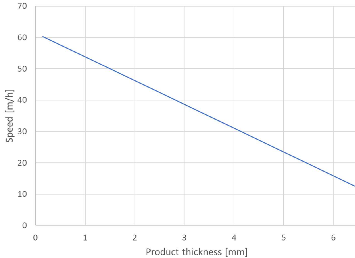
Performance for the vulcanization of rubber plates, Auma type 20 (Rotocure machine with heating drum diameter = 2.0 m)
