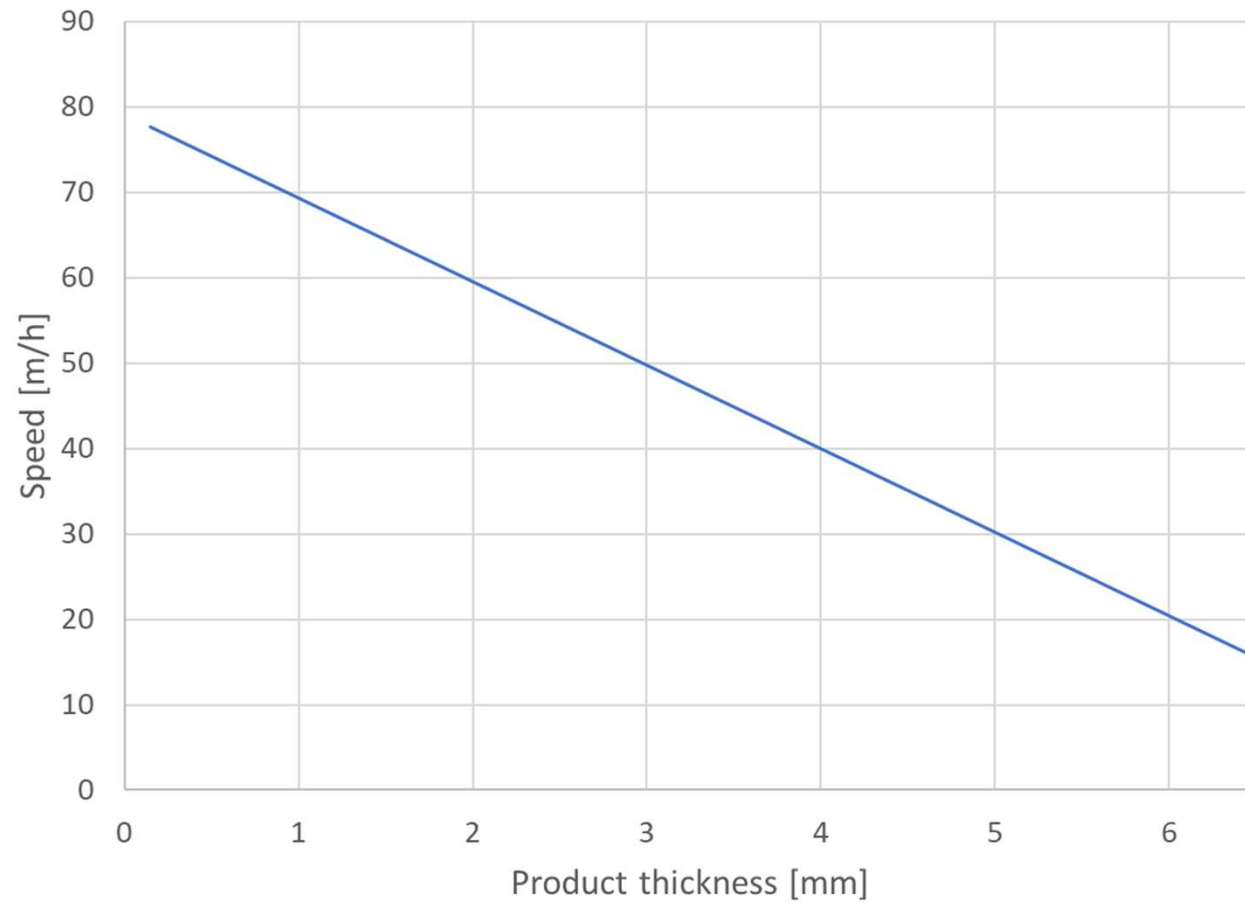
Performance for the vulcanization of rubber plates, Auma type 25 (Rotocure machine with heating drum diameter = 2.5 m)
