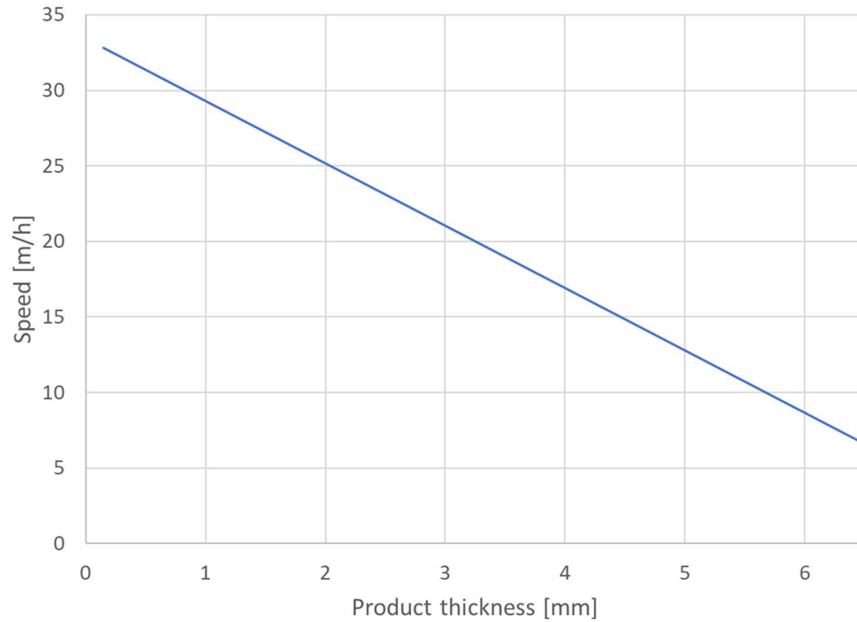
Performance for the vulcanization of rubber plates, Auma type 10 (Rotocure machine with heating drum diameter = 1.0 m)
