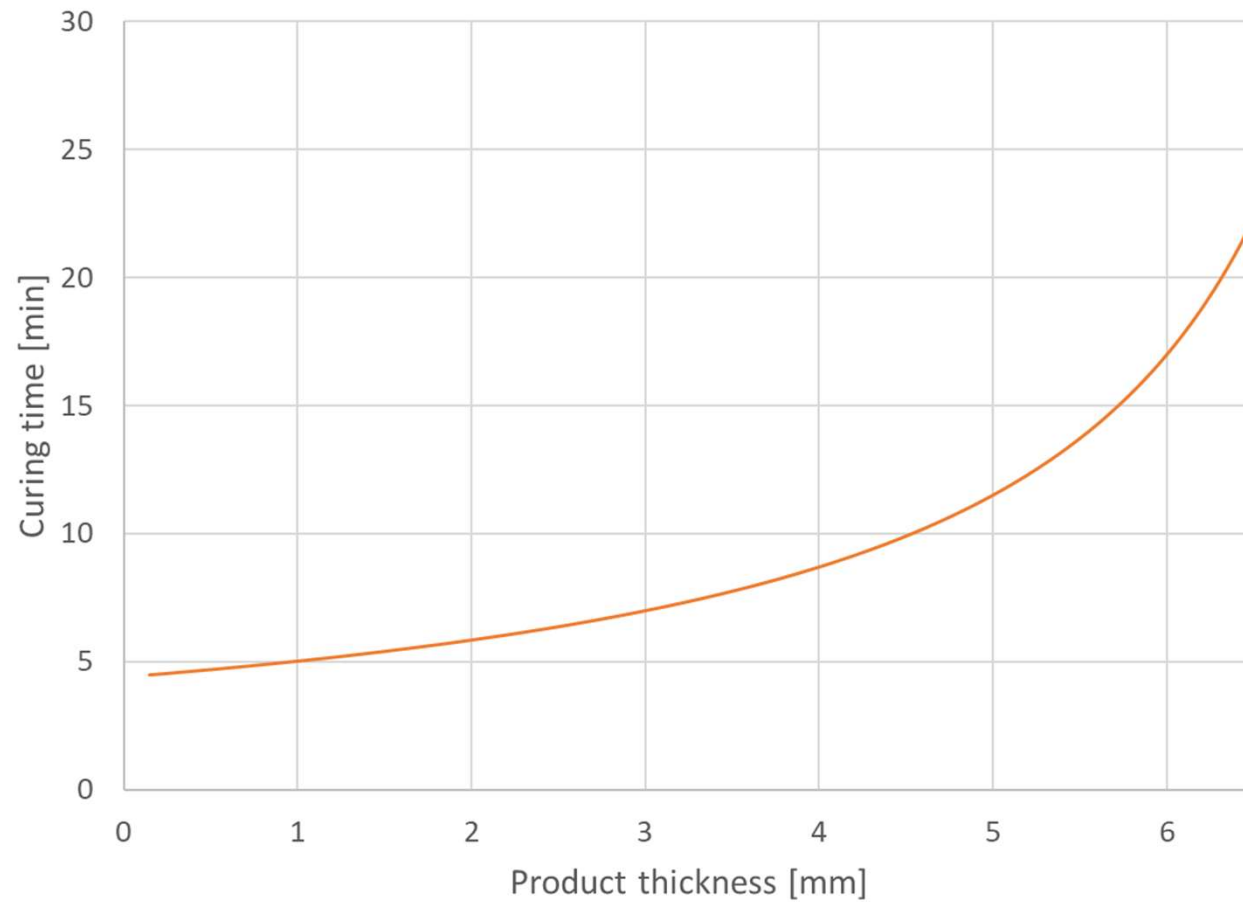
Curing times for the vulcanization of rubber plates, Auma type 20 (Rotocure machine with heating drum diameter = 2.0 m)
