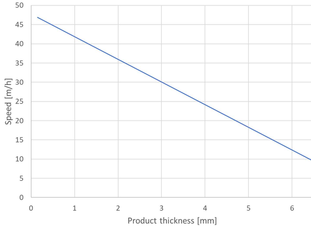
Performance for the vulcanization of rubber plates, Auma type 15 (Rotocure machine with heating drum diameter = 1.5 m)
